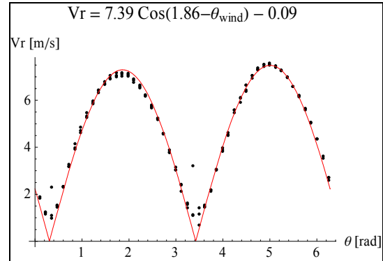
Figure 2 Example of result from a 3-second scan. The black points are the actual radial wind speed measurements. The red line is the fit function (given at the top of the figure).
