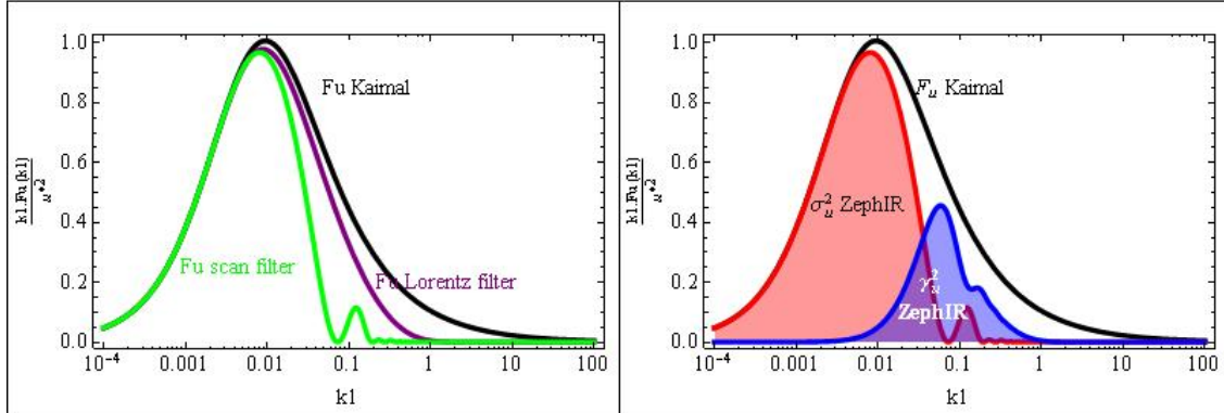
Figure 7 Stream wise component of the Kaimal spectrum (black) shown as a reference. Left: spectrum filtered with the Lorentzian filter (purple), spectrum filtered with the scan filter (green). Right: spectrum of 10 minutes stream-wise turbulence obtained from a cw conically scanning LiDAR (red), turbulence spectrum obtained with the high-pass filter modeling the turbulence unresolved by the conical scanning effect (blue), see equation (17). The spectra shown correspond to a focus height z=30m (then the circle diameter is 34.6m ), for a 3-second scan and z_r=0.0017z^2 ( z=r\cos(30^\circ) ).
